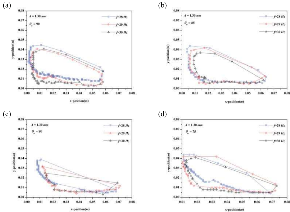
Fig. 3 Motion of intruder granular materials in containers under vibration with side wall angles of (a) \theta_w = 90^\circ , (b) \theta_w = 85^\circ , (c) \theta_w = 80^\circ , and (d) \theta_w = 75^\circ (at A = 1.30 mm and f = 28, 29 , and 30 Hz).
