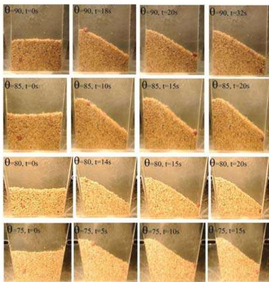
Fig. 4 Convection forming and segregation generated by container wall angles of \theta_w = 90^\circ, 85^\circ, 80^\circ , and 75^\circ degrees (at A = 1.30 mm, f = 28 Hz, and \Gamma = 4.102 ).
