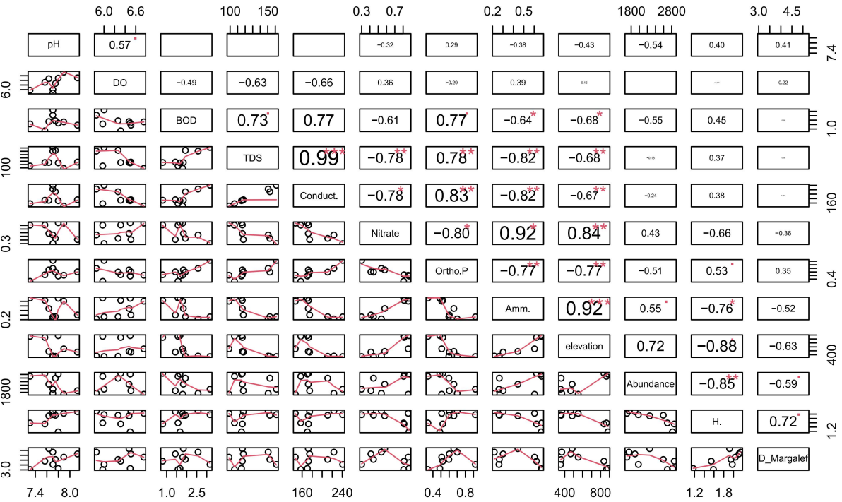
Fig. S1 Spearman's correlation between physicochemical parameters among sampling sites in Mae Ram River basin. * p < 0.05 , ** p < 0.01 , and *** p < 0.001 .
