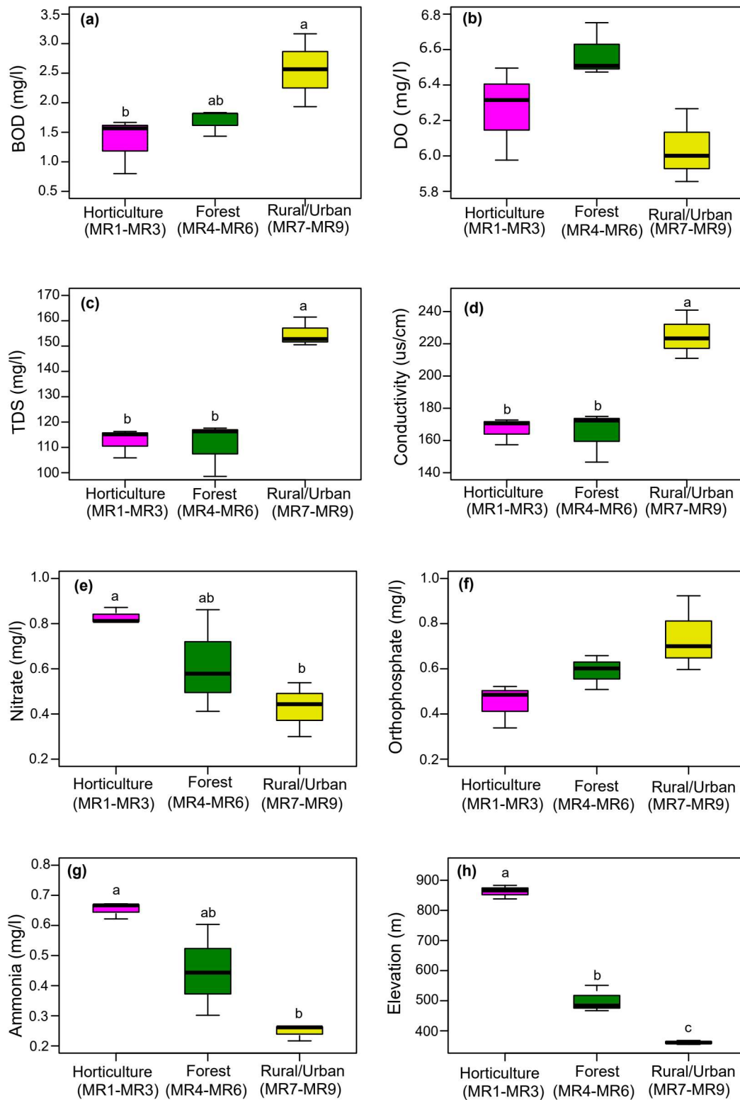
Fig. 2 Differences in environmental variables and land-use types of Mae Ram River; (a) Biochemical oxygen demand (BOD), (b) Dissolved oxygen (DO), (c) Total dissolved solid (TDS), (d) Conductivity, (e) Nitrate, (f) Orthophosphate, (g) Ammonia, and (h) Elevation. Letters indicate significant differences according to Tukey's test (except Elevation; Dunn's test). Bold horizontal lines represent medians, boxes represent interquartile ranges (25th–75th percentiles), and range bars show maximum and minimum values.
