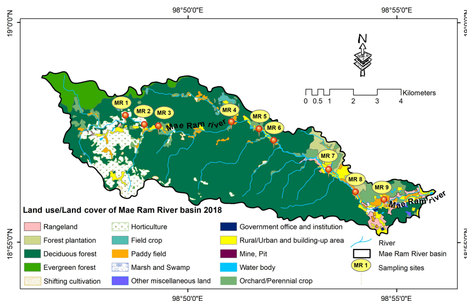
Fig. 1 Location of study sites at Mae Ram River basin.
