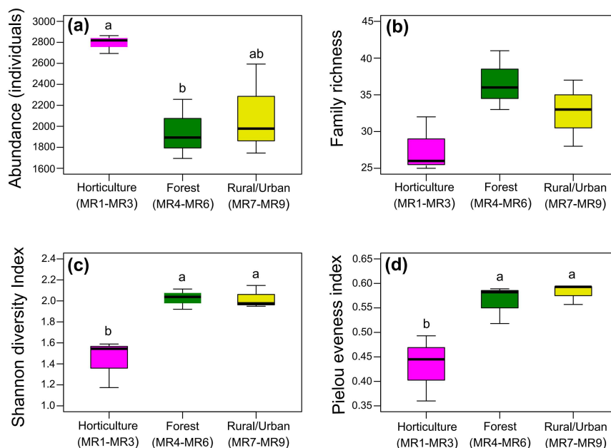
Fig. 3 Box plots of different land-use types and macroinvertebrate communities. (a) Abundance, (b) Family richness, (c) Shannon diversity, and (d) Pielou evenness. Letters indicate significant differences according to Tukey's test. Bold horizontal lines represent medians, boxes represent interquartile ranges (25th–75th percentiles), and range bars show maximum and minimum values.
